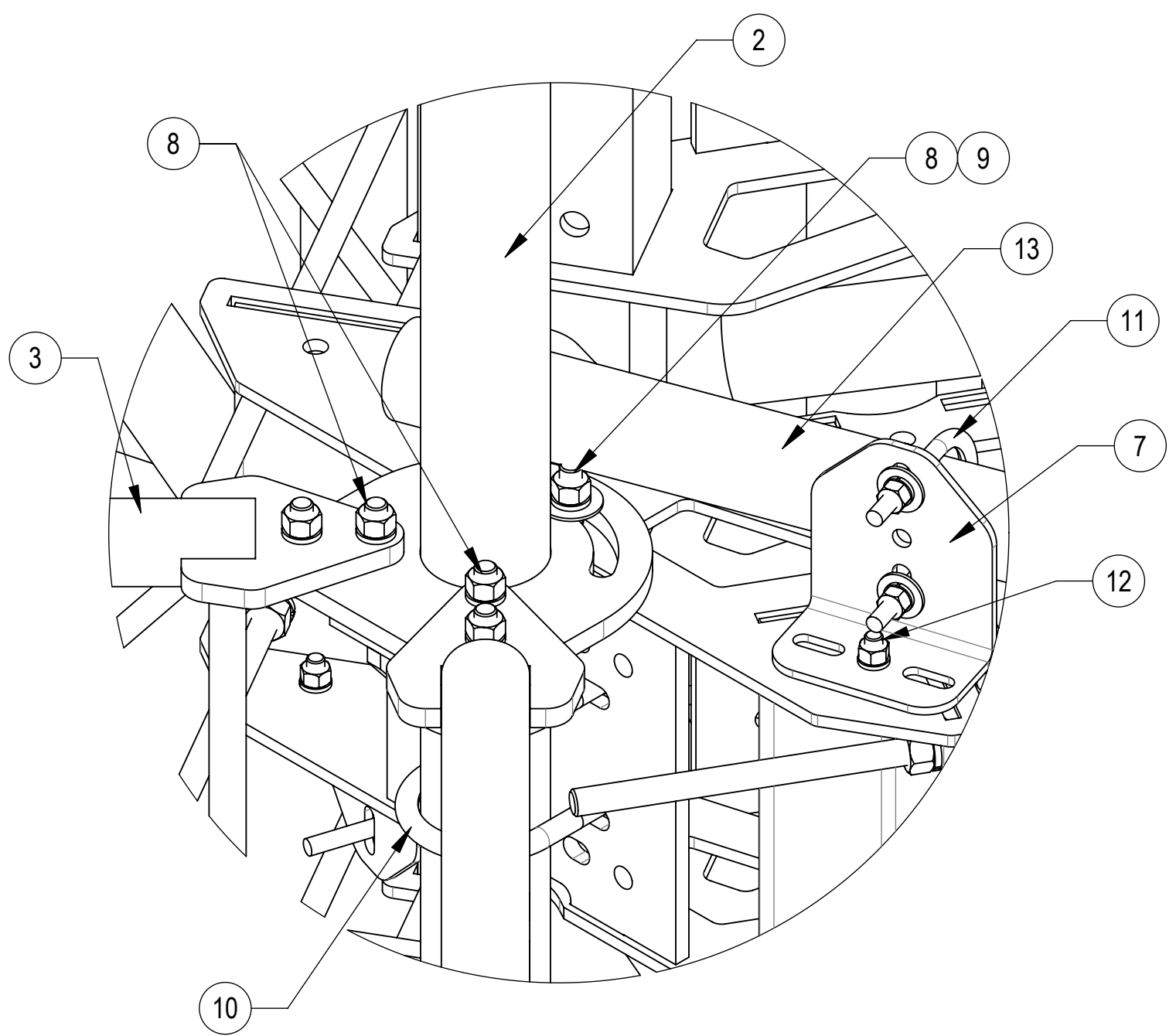
DETAIL B SCALE 1 : 4
