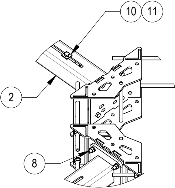
DETAIL C SCALE 2 : 25
