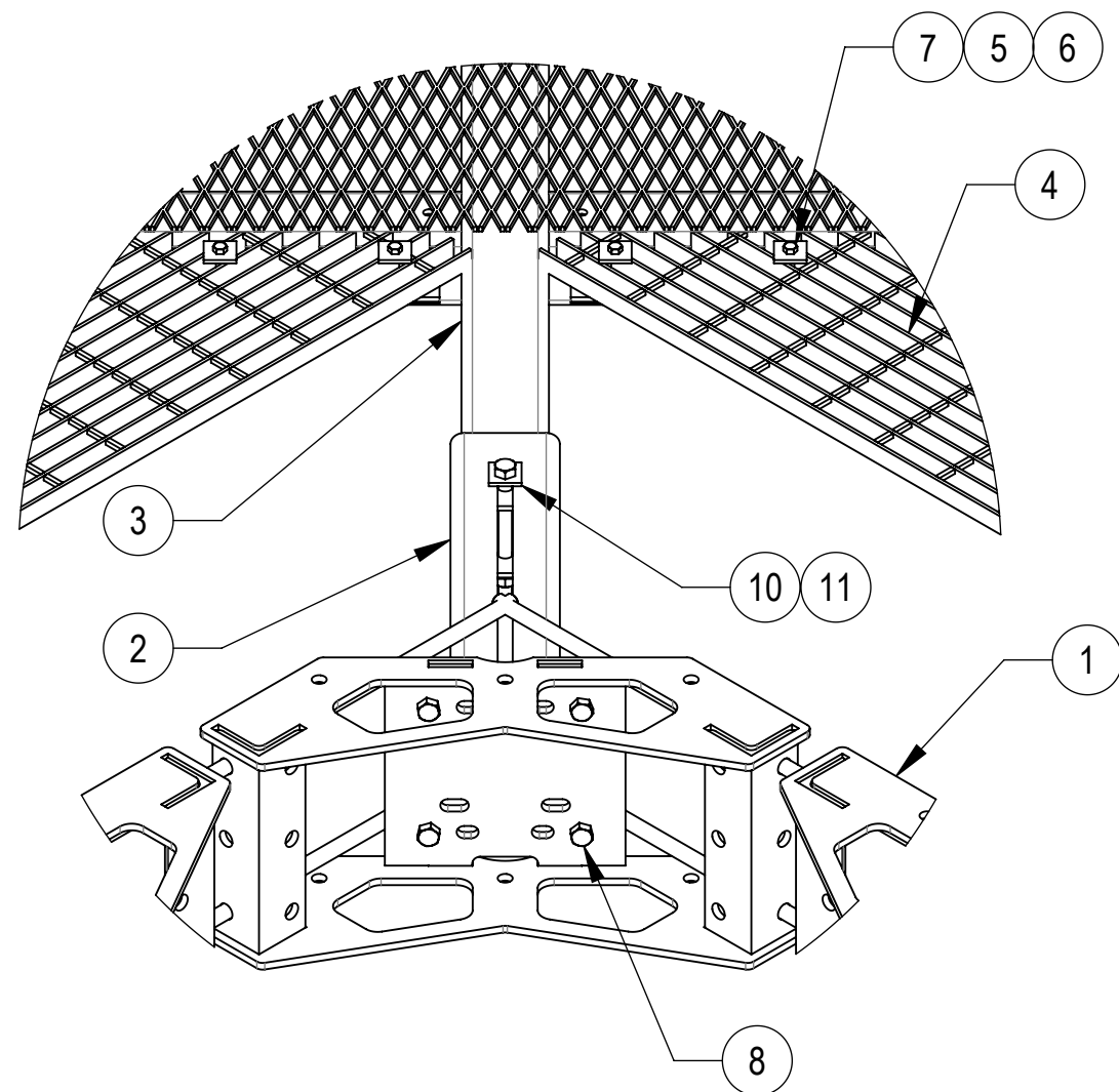
DETAIL A SCALE 1 : 9
